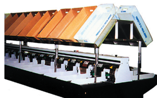
PTI Model
